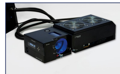
Remote radiator with 2x 120 mm fans for liquid cooling
